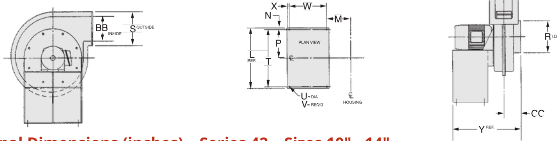
Principal Dimensions (inches) – Series 42 – Sizes 10" - 14"
