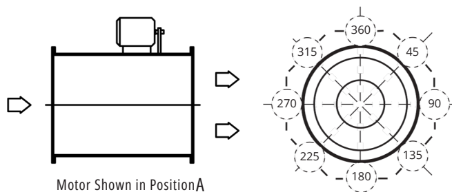
View Facing Outlet
