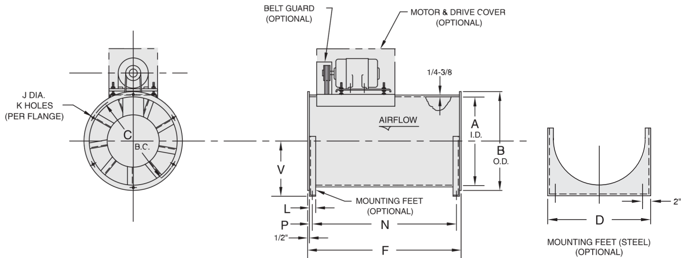
Principal Dimensions (inches) – Series 40 – Sizes 12" – 60"
