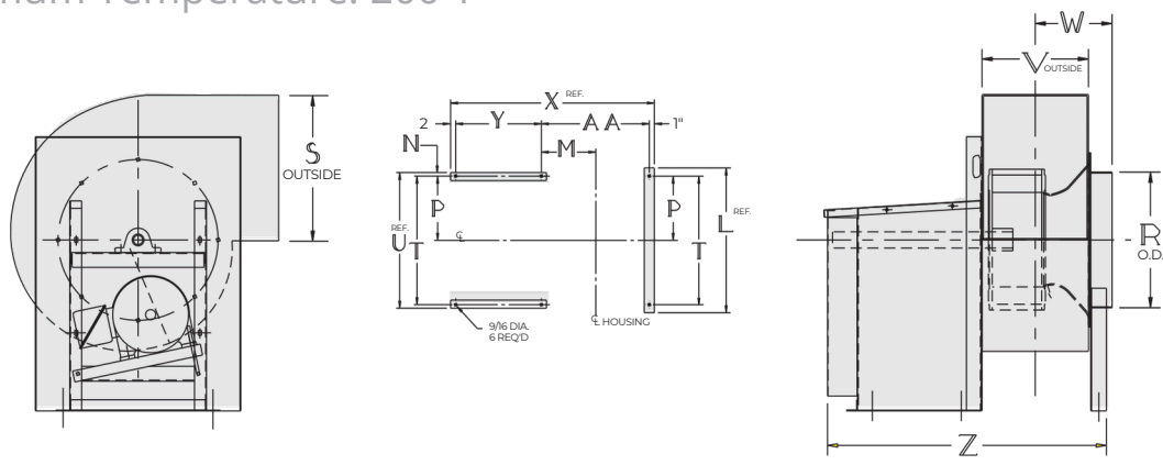
Principal Dimensions (inches) – Series 41U – Sizes 12" – 24"
